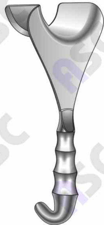
De Lee Universal Retractor 32-3235-24 24 cm / 9 1/2" Blade 2 1/4" x 2"
