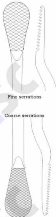
Miller-Colburn 23-3301-21 21.5 cm / 8½" Double ended, 13 mm width Cross serrations, for rapid shaping of bone
